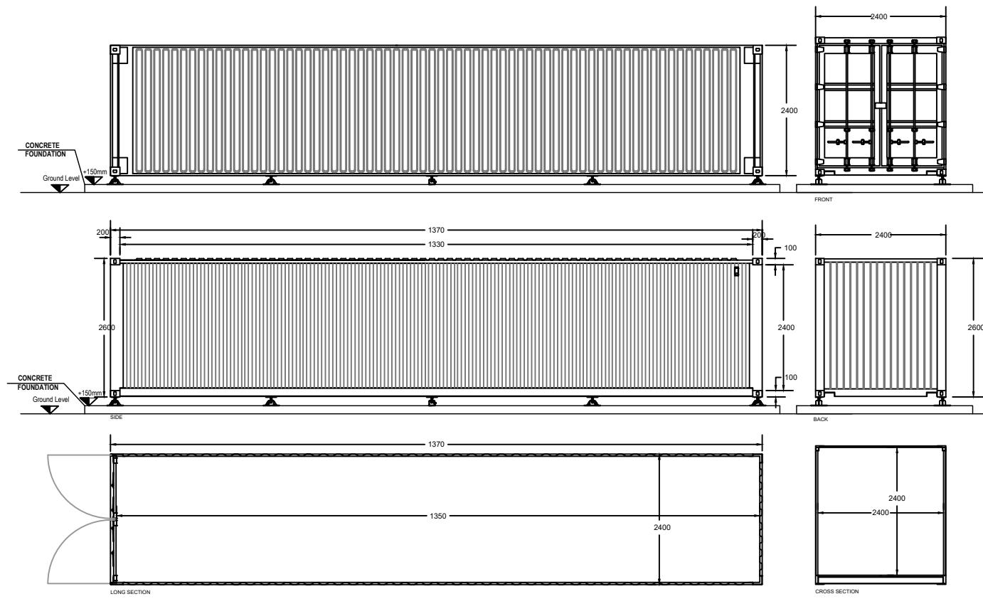
Spare parts container details
